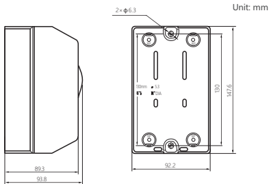
Figure 6 Overall and installation dimensions of NS2-MC
