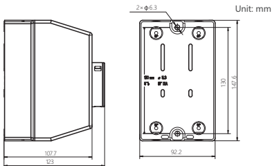
Figure 8 Overall and installation dimensions of WPB-1
