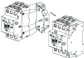
Figure 13 Assembly method for NS2-SH
