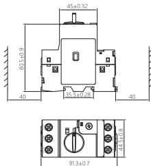
Figure 3 Overall and installation dimensions of NS2-25X\NS2-32X
