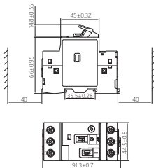
Figure 2 Overall and installation dimensions of NS2-25\NS2-32
