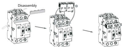
Figure 9 Assembly method for NS2-AE
