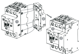
Figure 12 Assembly method for NS2-UV
