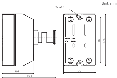
Figure 7 Overall and installation dimensions of NS2-MC01
