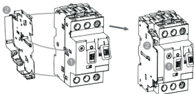
Figure 10 Assembly method for NS2-AU
