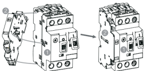
Figure 11 Assembly method for NS2-FA
