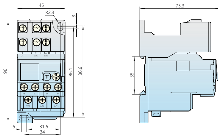
NXR-12 + MB-1
