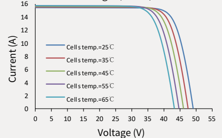
Current-Voltage (610W)
