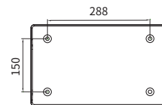
Dimension drawing
