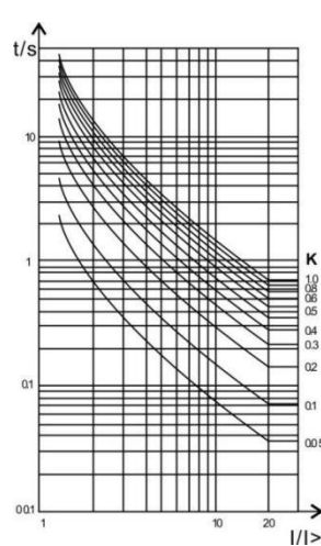
IDMT Very Inverse
