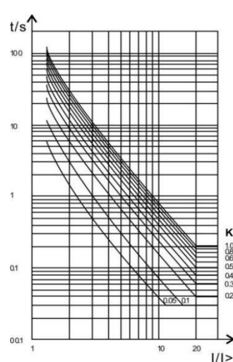
IDMT Extremely Inverse
