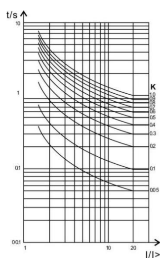
IDMT Inverse 1.3/10
