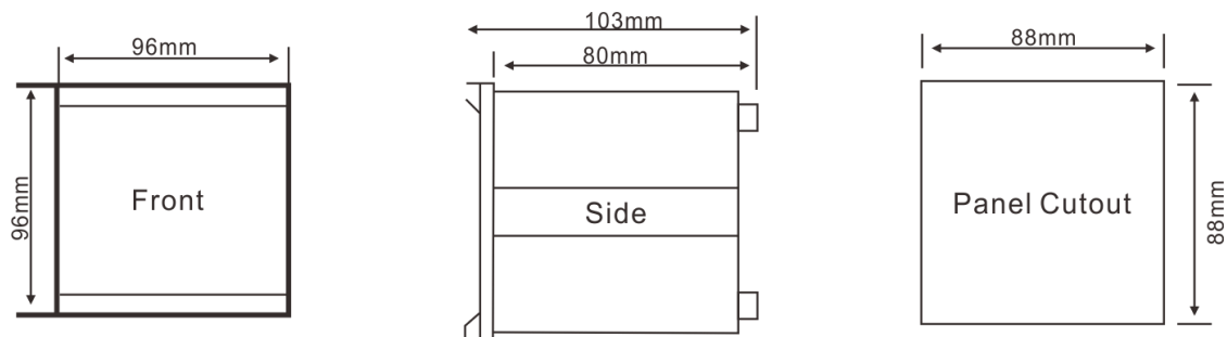
Figure3: Case Dimension
