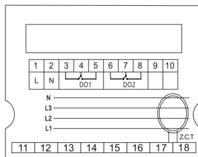
Figure4: Connection Diagram
