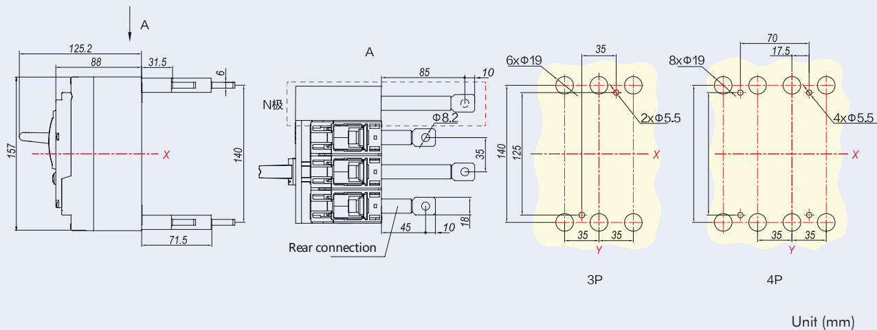
NM8N-250 Rear connection (3P/4P)
