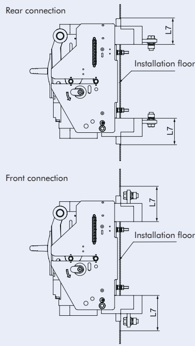
DIN-rail mounting
