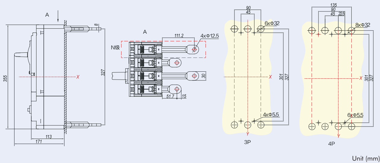
NM8NL-400/630 Rear connection
