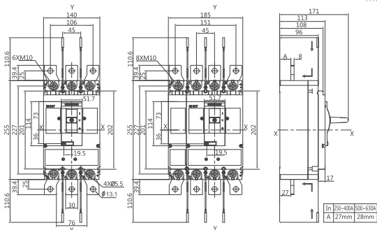
Diagram 3. NM8N(DC)-400, 630
