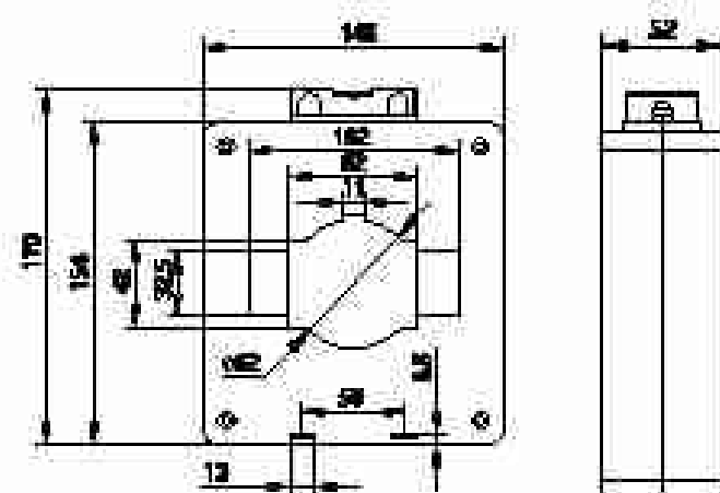
External ground current transformer
