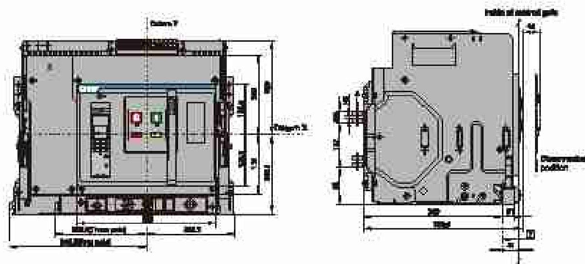
Side view
