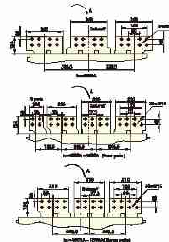
Breaker size and terminal
