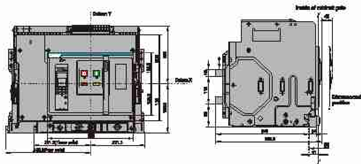
Side view
